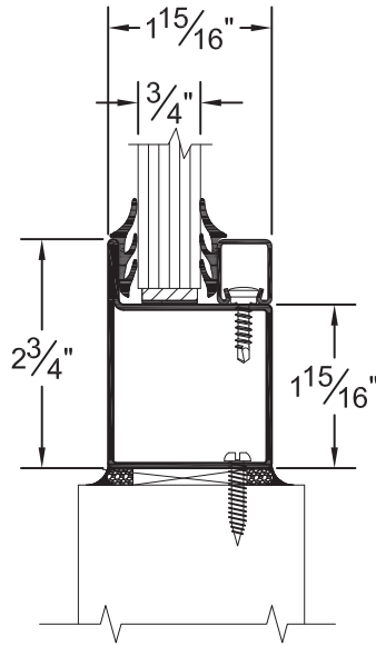
TYPICAL VDS LITE PERIMETER DETAIL
