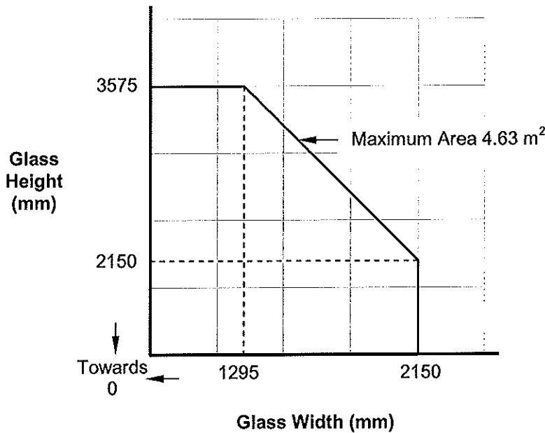
Figure 6. Maximum Permitted Glass Dimensions
