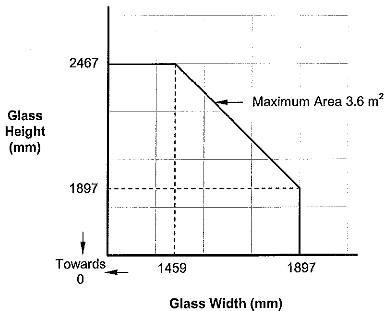
Figure 7. Maximum Permitted Glass Dimensions
